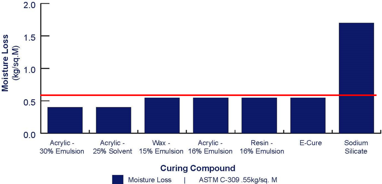
Moisture Loss of Concrete Curing Compounds: (Applied @ 200 sq. ft./gal.; measured 72 hours after application)
